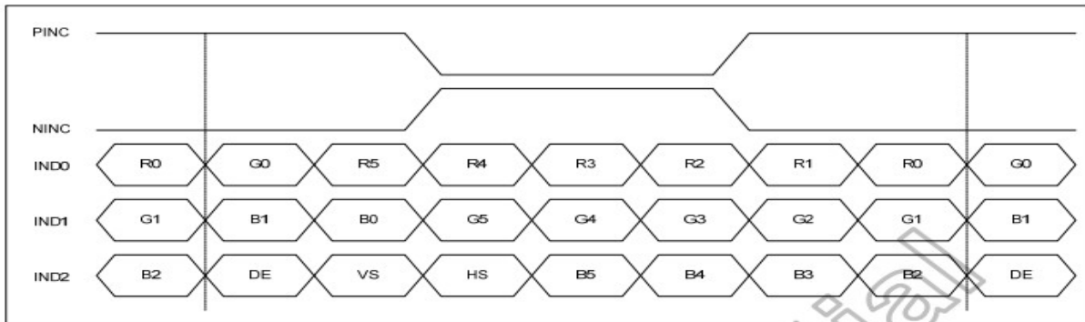
6-bit LVDS input
